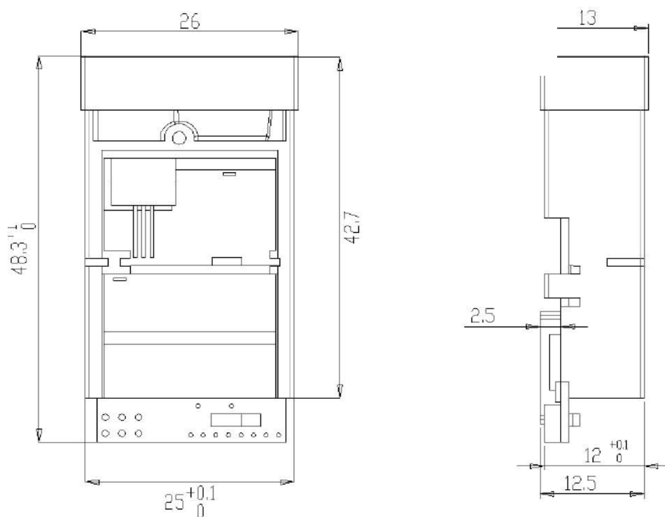
Figure 3-1 Mechanical Size
